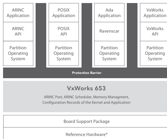
Figure 2: IMA design with VxWorks 653 Platform
